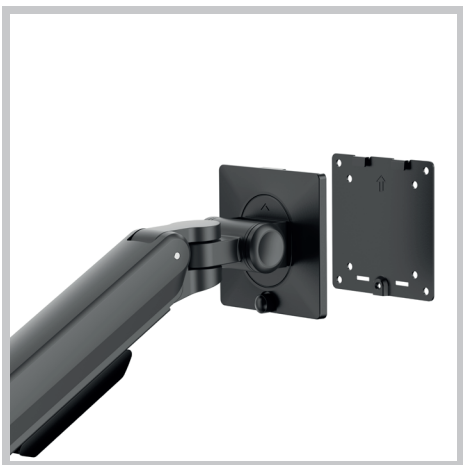
Quick-release VESA plate for easy installation and removal.
